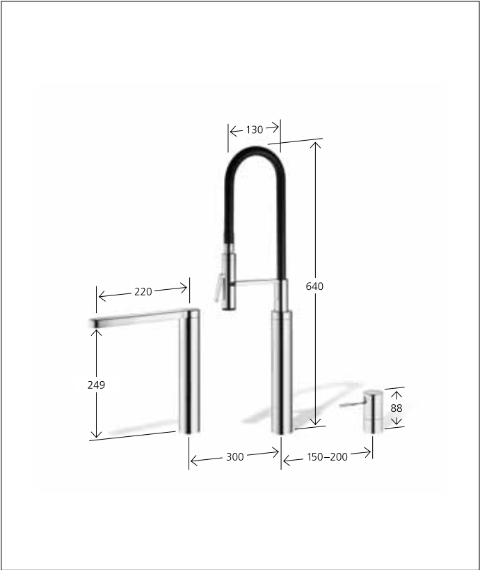
Lever mixer highflex® patented spring hose technology 3-hole swivel spout 360° professional spray 360° turn 10.153.423.000FL all chrome A 220
