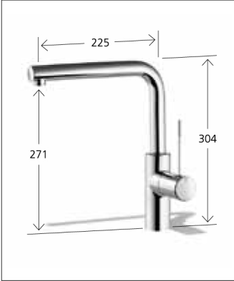
Lever mixer lever installation possible on the right or left side swivel spout 360° 10.151.013.000FL all chrome A 225
