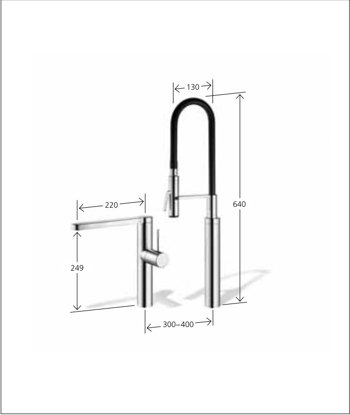
Lever mixer highflex® patented spring hose technology 2-hole swivel spout 360° professional spray 360° turn 10.152.423.000FL all chrome A 220
