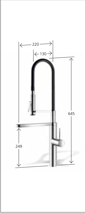
Lever mixer highflex® patented spring hose technology lever installation possible on the right or left side swivel spout 360° professional spray 360° turn 10.151.423.000FL all chrome A 220 10.151.423.700FL stainless steel A 220
