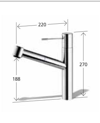
Lever mixer pull-out spray with KWC jetClean up to 700 mm pull-out length hose guide swivelling 105° 10.151.033.000FL all chrome A 220 10.151.033.700FL stainless steel A 220
