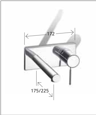
Lever mixer fixed spout 11.152.033.000 all chrome A 175 11.152.034.000 all chrome A 225 To be ordered separately: unit for concealed installation ½" 39.151.400.931
