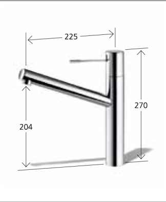
Lever mixer swivel spout 270° 10.151.023.000FL all chrome A 225 10.151.023.700FL stainless steel A 225
