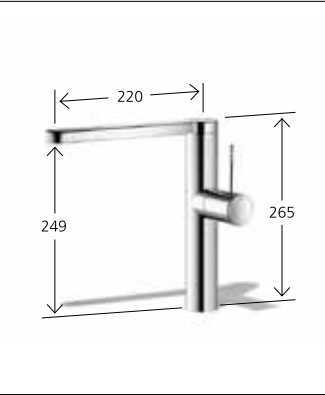
Lever mixer lever installation possible on the right or left side swivel spout 360° 10.151.413.000FL all chrome A 220 10.151.413.700FL stainless steel A 220
