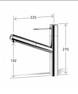
Lever mixer pull-out aerator up to 700 mm pull-out length hose guide, swivelling 105° 10.151.113.000FL all chrome A 225 10.151.113.700FL stainless steel A 225
