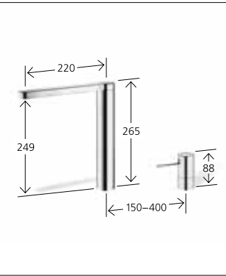
Lever mixer 2-hole swivel spout 360° 10.152.413.000FL all chrome A 220
