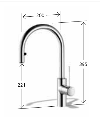
Lever mixer lever installation possible on the right or left side pull-out aerator covered up to 700 mm pull-out length hose guide swivelling 360° 10.151.102.000FL all chrome A 200 10.151.102.700FL stainless steel A 200
