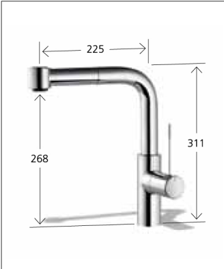
Lever mixer lever installation possible on the right or left side pull-out spray with KWC jetClean up to 700 mm pull-out length hose guide swivelling 360° 10.151.003.000FL all chrome A 225
