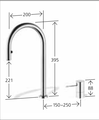
Lever mixer 2-hole pull-out aerator covered hose guide swivelling 360° 10.152.322.000FL all chrome A 200
